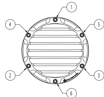
FIG B TORQUE SEQUENCE
