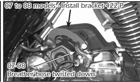
FIGURE 2 07 to 08 models - Install bracket 422-P
